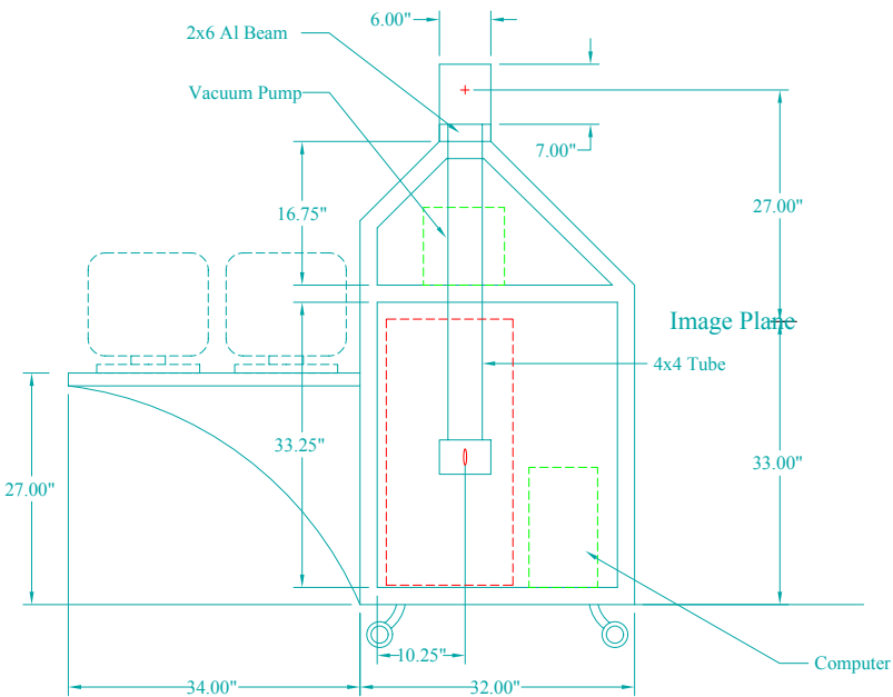
Right Side
