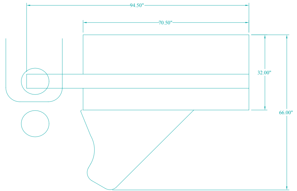
Plan View
