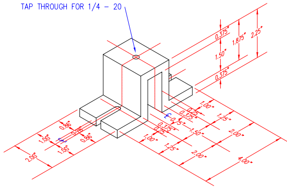
RISER FOR CYLINDRICAL LENSES
