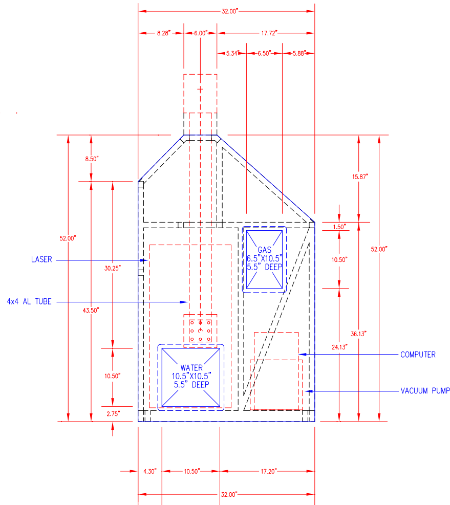
GAS & WATER LOCATIONS SCALE: 1 1/2" = 1'-0"
