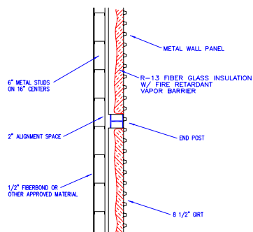
WALL DETAIL "W-10"
