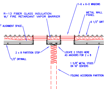
WALL DETAIL "W-2"
