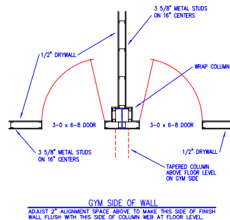
WALL DETAIL "W-3"
