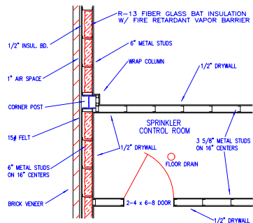
WALL DETAIL "W-5"
