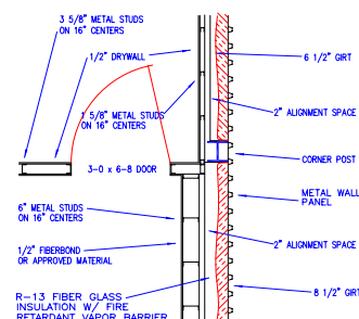
WALL DETAIL "W-8"
