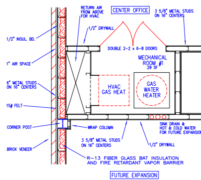
WALL DETAIL "W-11"
