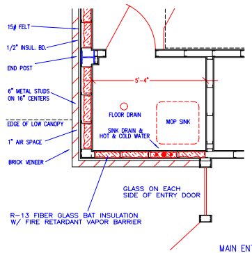
WALL DETAIL "W-9"
