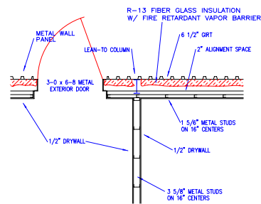
WALL DETAIL "W-3"
