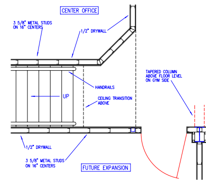
WALL DETAIL "W-12"
