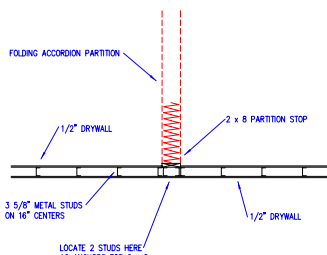
WALL DETAIL "W-2"
