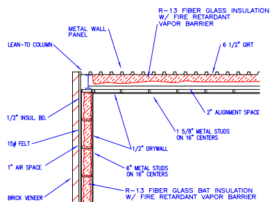
WALL DETAIL "W-1"
