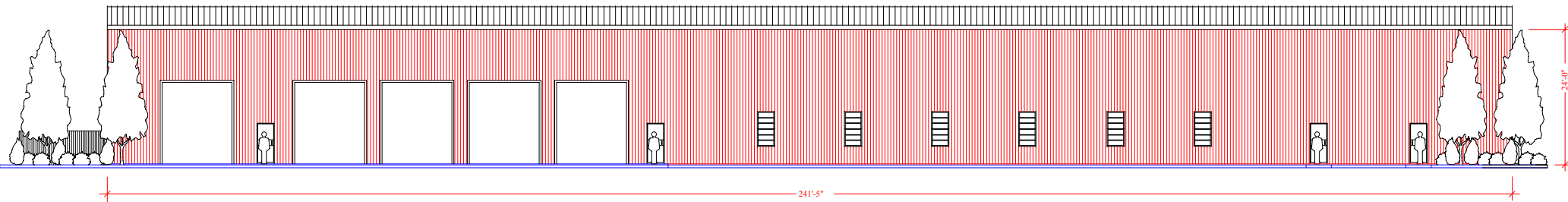
LEFT SIDE ELEVATION SCALE: 3/32" = 1'-0"
