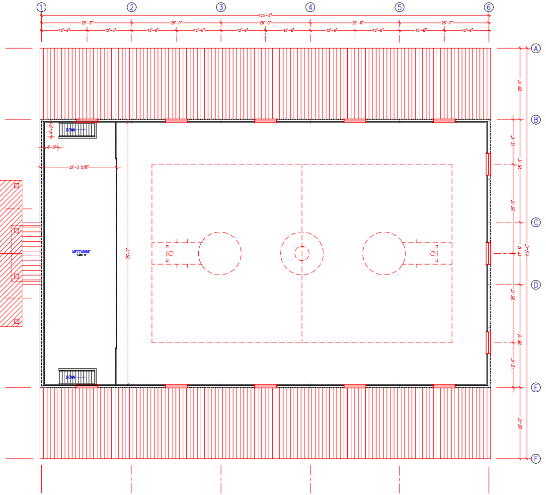
MEZZANINE LEVEL PLUMBING PLAN SCALE: 1/8" = 1' - 0"
