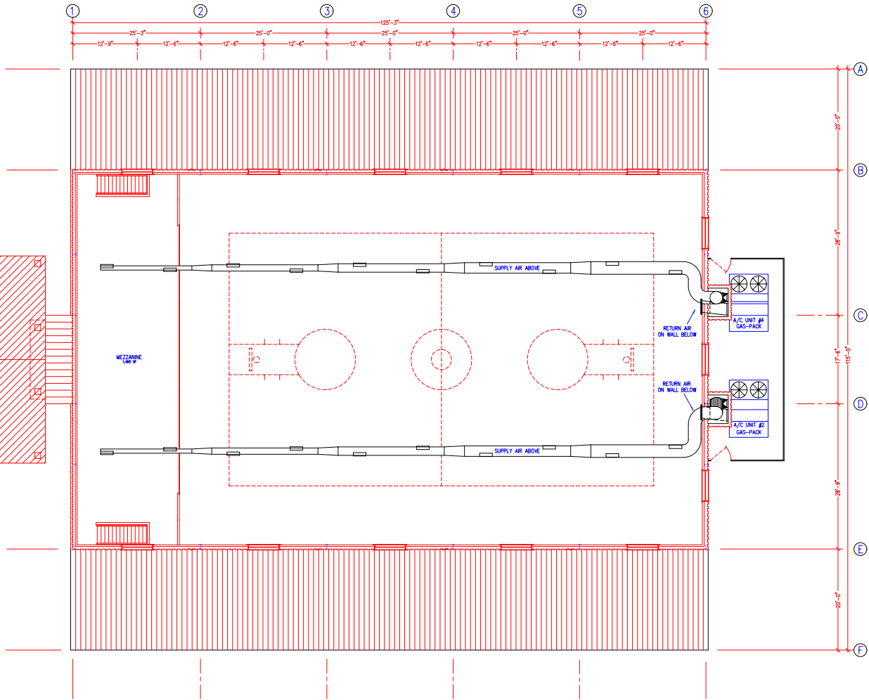
MEZZANINE LEVEL MECHANICAL PLAN SCALE: 1/8" = 1' - 0"
