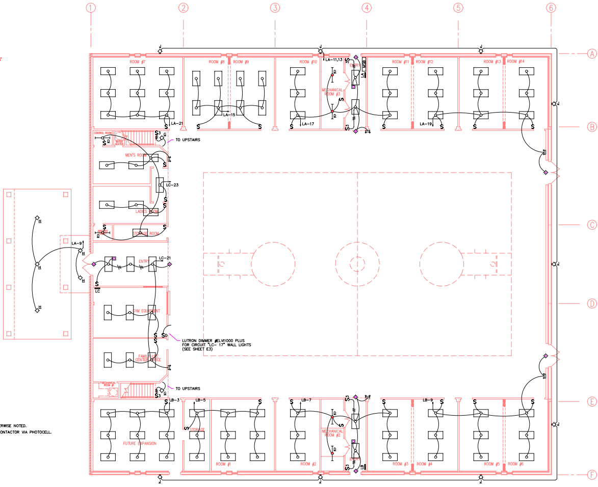
FIRST LEVEL LIGHTING PLAN SCALE: 1/8" = 1' - 0"
