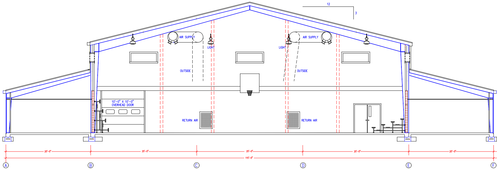
SECTION "A-A" (Looking North) SCALE: 1/4" = 1'-0"
