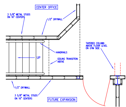
WALL DETAIL "W-12"
