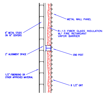
WALL DETAIL "W-10"
