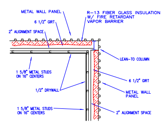
WALL DETAIL "W-4"
