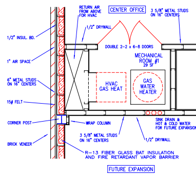
WALL DETAIL "W-11"
