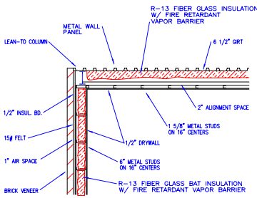
WALL DETAIL "W-1"
