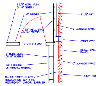
WALL DETAIL "W-8"
