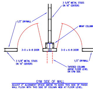
WALL DETAIL "W-7"
