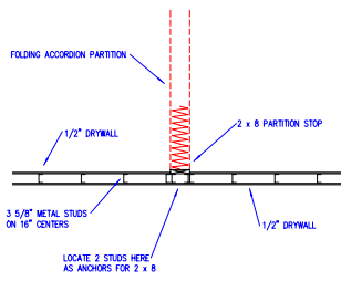
WALL DETAIL "W-2"
