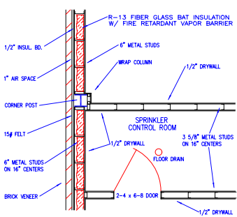
WALL DETAIL "W-5"
