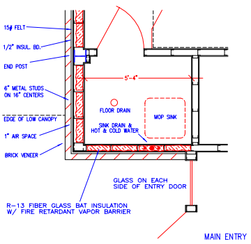
WALL DETAIL "W-9"
