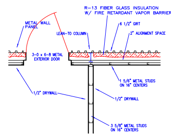
WALL DETAIL "W-3"
