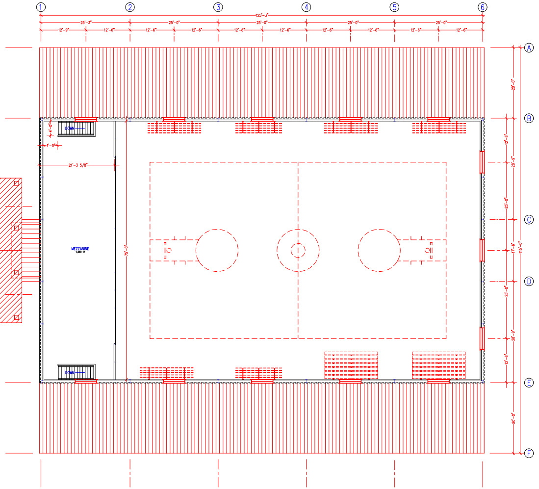
MEZZANINE LEVEL FLOOR PLAN SCALE: 1/8" = 1' - 0"
