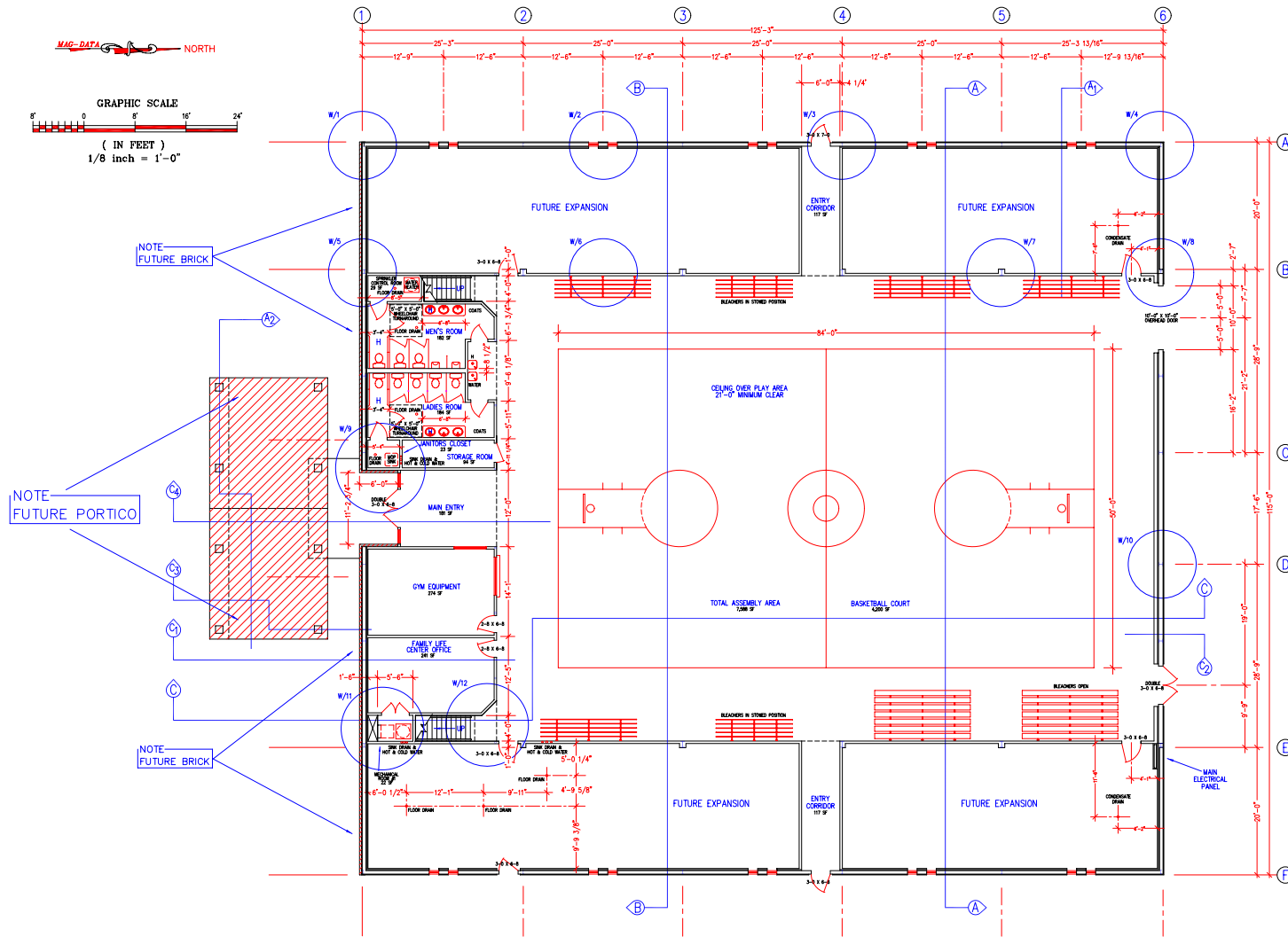
1st LEVEL FLOOR PLAN SCALE: 1/8" = 1' - 0"
