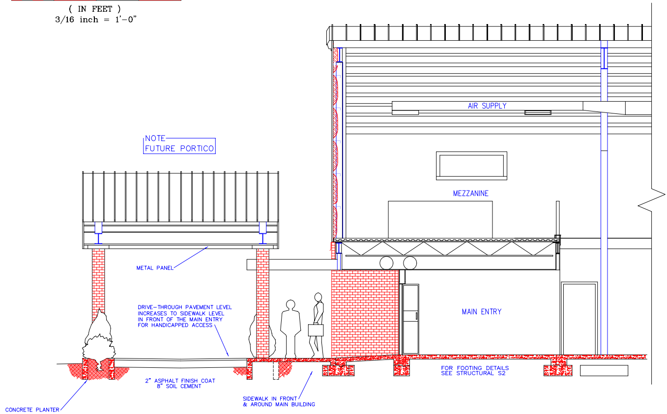
SECTION "C4" (THROUGH ENTRY LOOKING WEST) SCALE: 3/8" = 1'-0"
