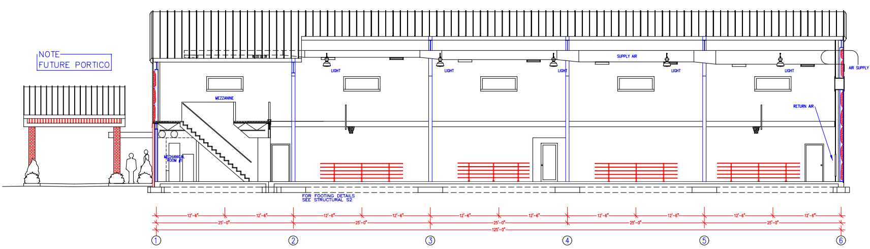
SECTION "C-C" (Looking West) SCALE: 3/16" = 1'-0"
