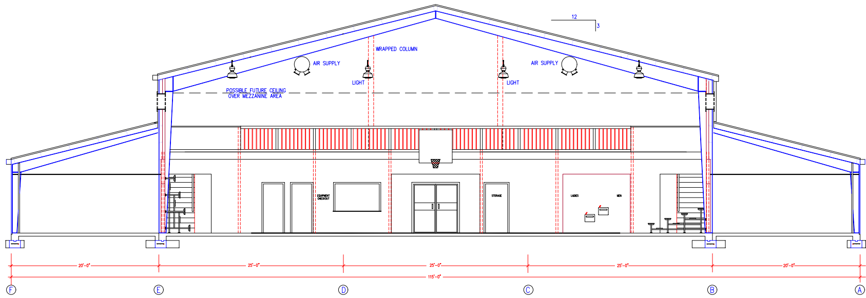
SECTION "B-B" (Looking South) SCALE: 1/4" = 1'-0"
