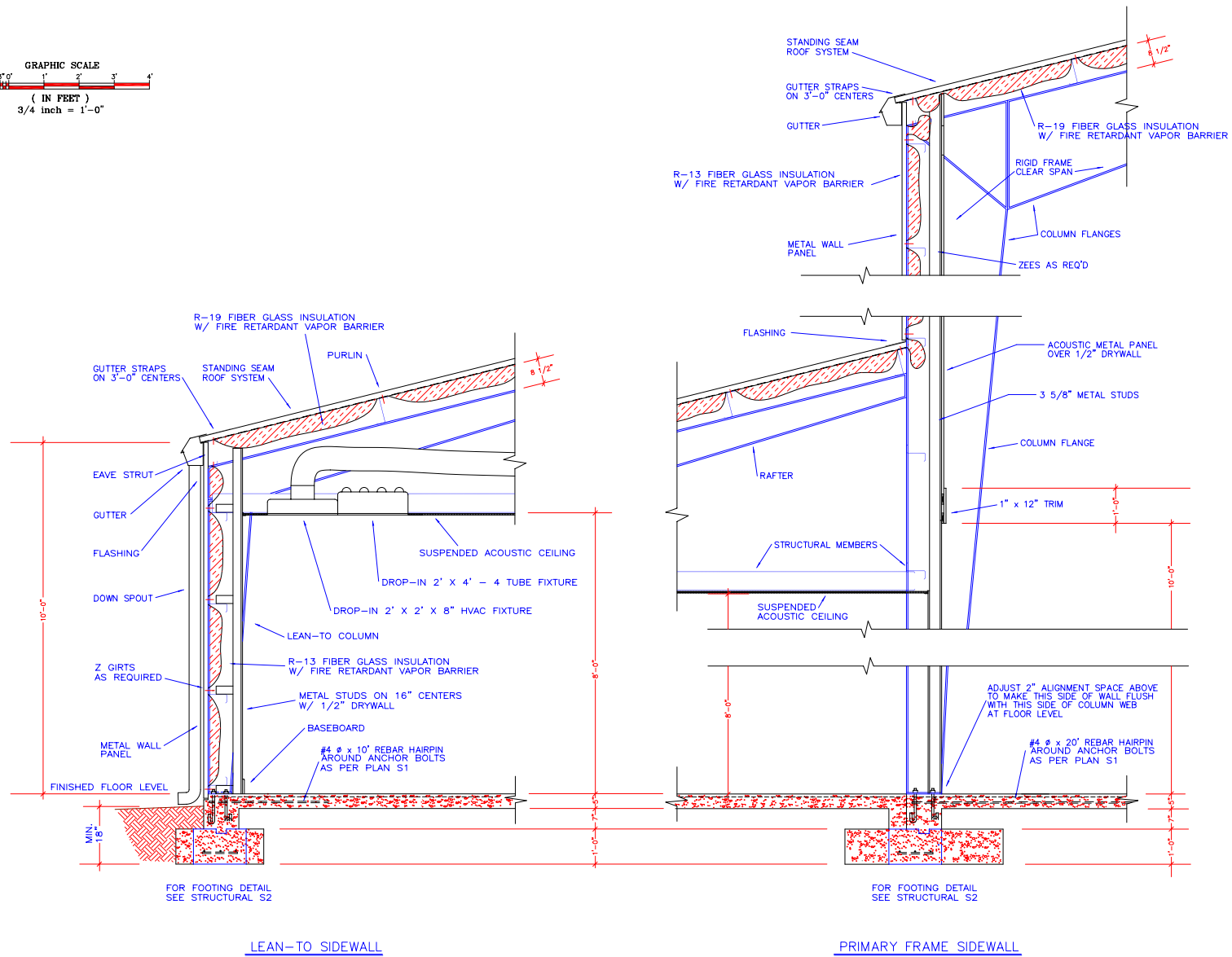
SECTION "A1" (LOOKING NORTH) SCALE: 3/4" = 1' - 0"
